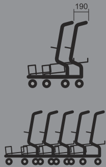
MULTI-BASKET TROLLEY
