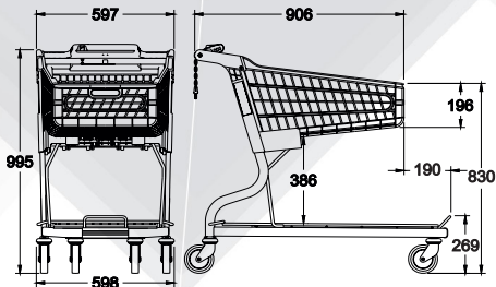
CPGGSP9008 22 kg.
